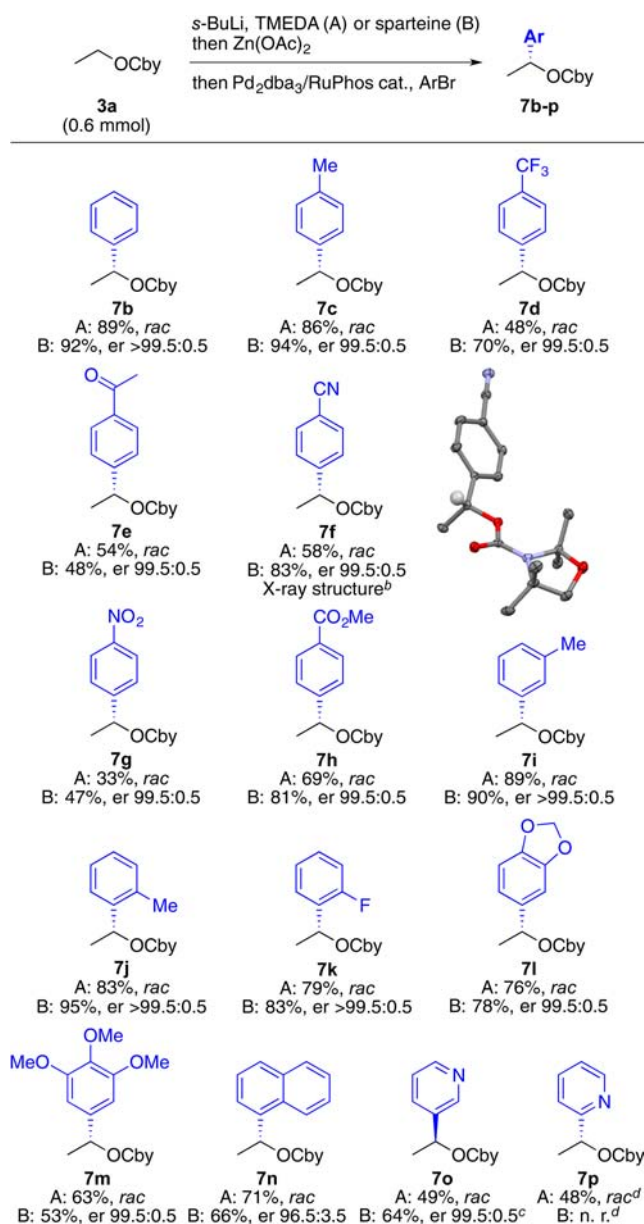
Scheme 2. Scope of the Racemic and Enantioselective \alpha -Arylation Reactions in Aryl Bromide a
