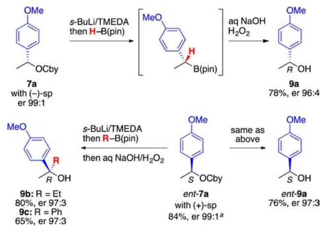
Scheme 4. Synthesis of Enantioenriched Secondary and Tertiary Alcohols via Aggarwal's Lithiation–Borylation Methods
