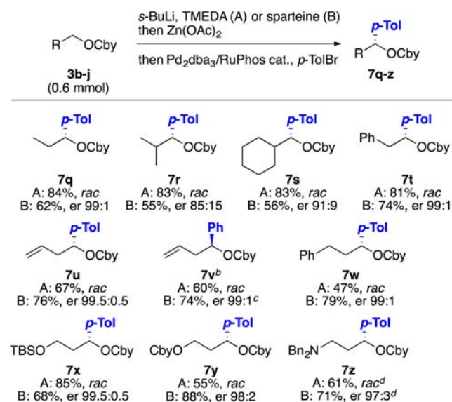
Scheme 3. Scope of the Racemic and Enantioselective \alpha -Arylation Reactions in Carbamate a
